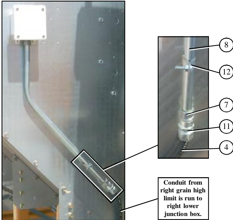
Right grain high limit thermostat enclosures.
